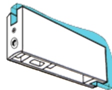
Fig. 500 Bottom Pivot Patch Fitting
